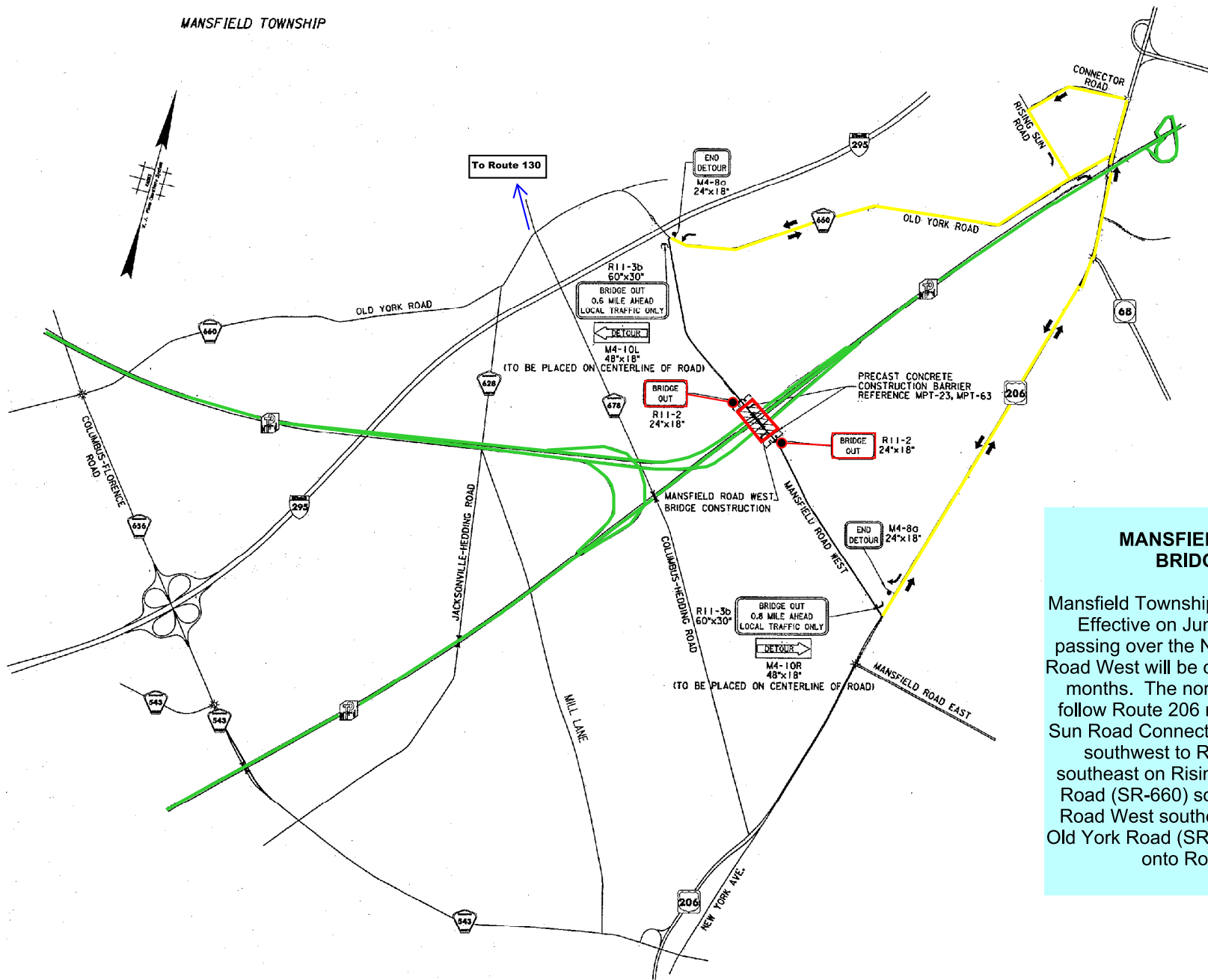
MANSFIELD ROAD WEST DETOUR STAGES 1-3
